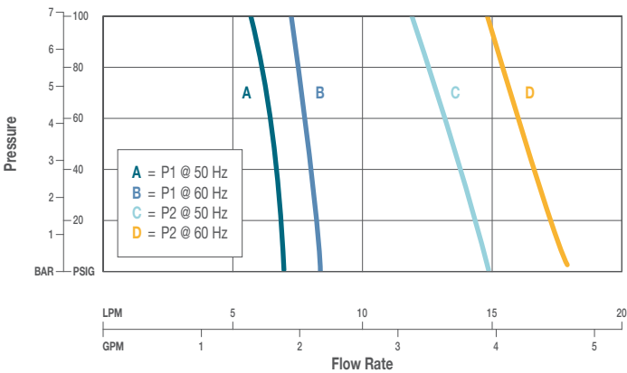
P5 Pump
