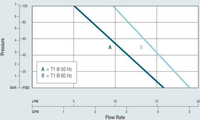
T1 Pump
