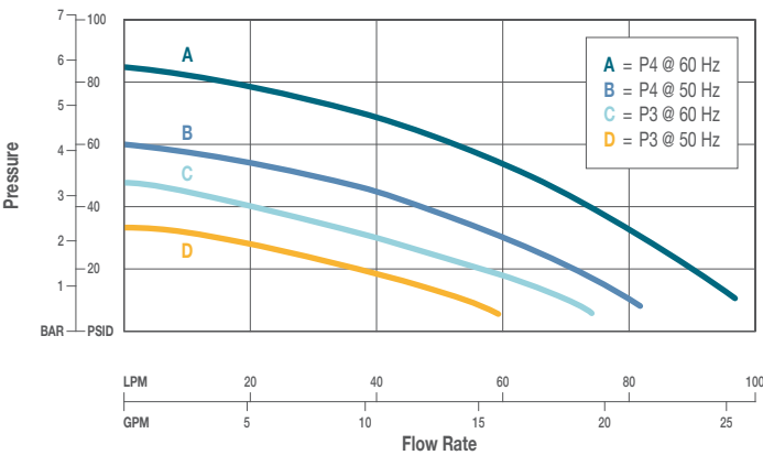
T5 Pump
